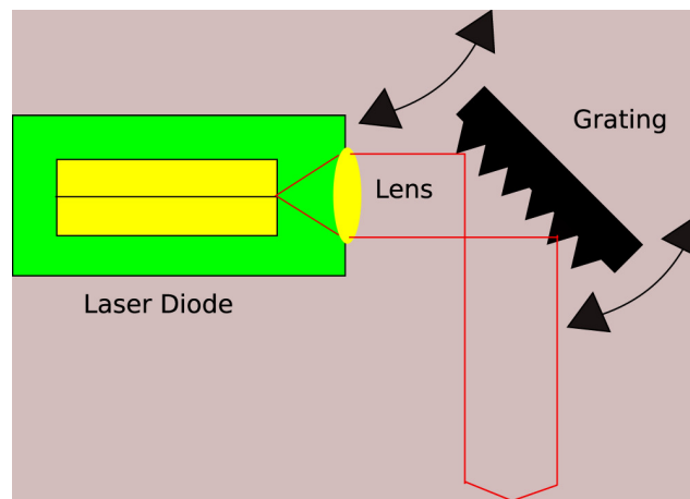
FIGURE 3.15: The Littrow configuration.
