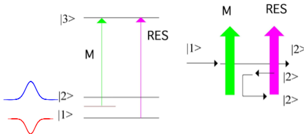
FIGURE 1.1: The simple model of a one-way barrier. The first laser beam M is tuned to the blue of the atomic transition |2\rangle \rightarrow |3\rangle and creates a repulsive barrier for atoms in state |2\rangle , but an attractive potential for atoms in state |1\rangle . The second laser beam RES is tuned to the atomic resonance |1\rangle \rightarrow |3\rangle and pumps the atoms from |1\rangle to |2\rangle . Adapted from [18].
