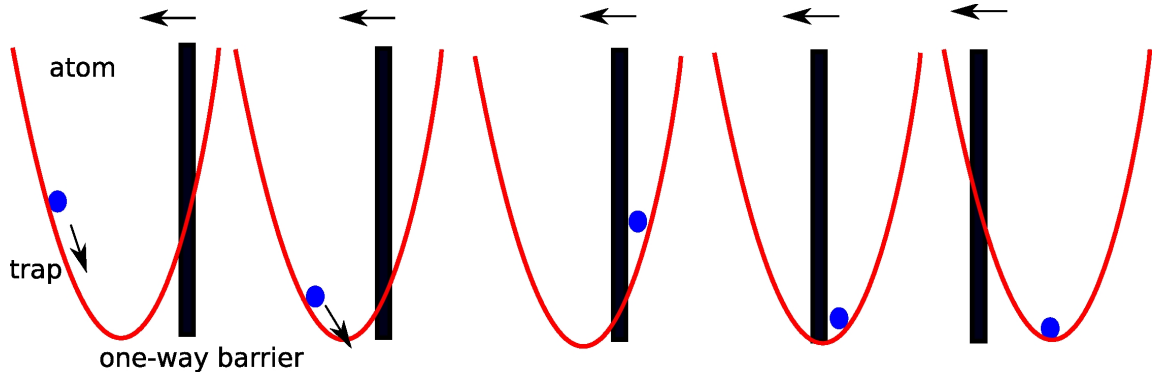
FIGURE 4.2: The schematic representation of the single-photon cooling method based on a one-way barrier. The atoms can pass the one-way barrier from left to right. The sequence of the 5 figures from left to right denotes the time evolution of the one-way barrier sweeping. Adapted from [72].
