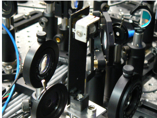
FIGURE 3.23: The mechanical shutter used for the pyramid MOT laser. It is mounted near the focus of a telescope system.
