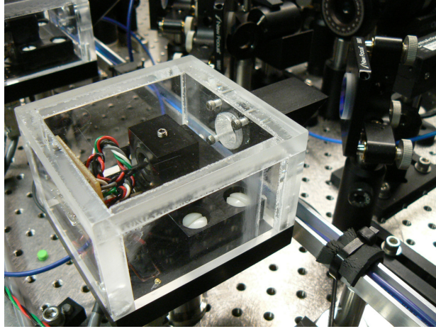
FIGURE 3.20: A slave laser. It shows the laser diode holder, the electrical connections and the housing with an optical window at Brewster's angle.
