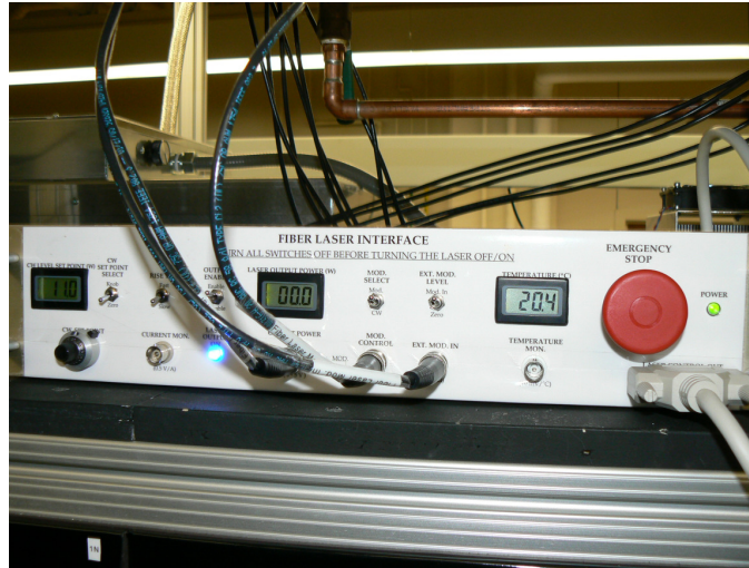
FIGURE 3.25: The fiber laser control box, which controls the fiber laser and acts as a modulation interface.
