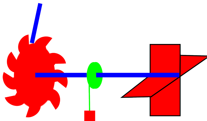
FIGURE 1.2: Feynman’s ratchet.
