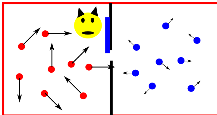
FIGURE 1.3: Maxwell's demon.
