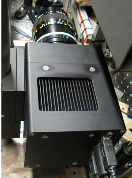
FIGURE 3.27: The MicroLine CCD camera equipped with a macro lens used to image atoms.
