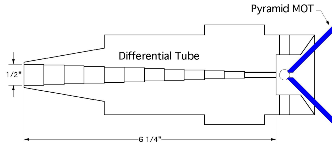
FIGURE 3.8: The differential pumping tube. The differential pumping tube has a low conductance of \sim 0.05 L/s. It connects the pyramid MOT vacuum chamber and the science vacuum chamber, in which the magnitudes of pressure have 3 orders difference. Adapted from a mechanical drawing by D. Steck.
