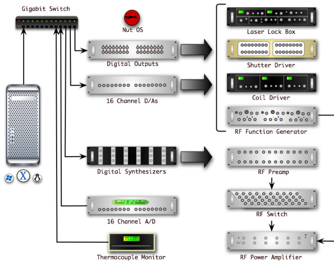
FIGURE 3.30: The structure of ZOINKS. The system includes a computer, Ethernet boards, UTBus-Ethernet interface boards, digital boxes, analog boxes, DDS, thermocouple monitors, and some other equipments that perform the experimental tasks, such as shutter driver, coil driver, RF function generator, etc. Adapted from [68].
