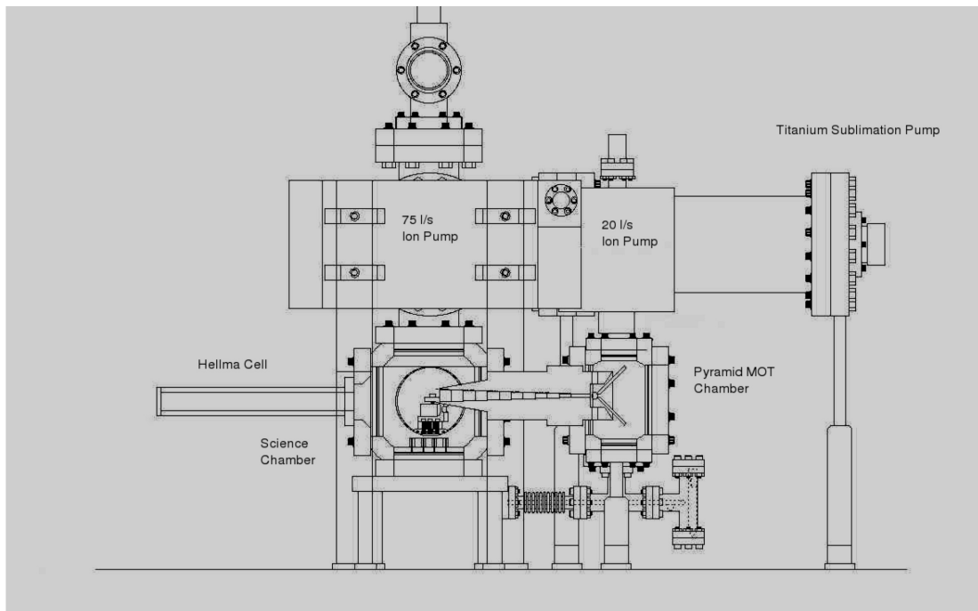
FIGURE 3.5: The mechanical drawing of the vacuum system. The picture shows the Hellma cell, science chamber, differential pumping tube, two ion pumps, titanium sublimation pump, getter pumps, and pyramid MOT vacuum chamber. Adapted from a drawing by D. Steck.
