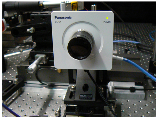
FIGURE 3.29: The Petcam works as an inexpensive beam profiler.
