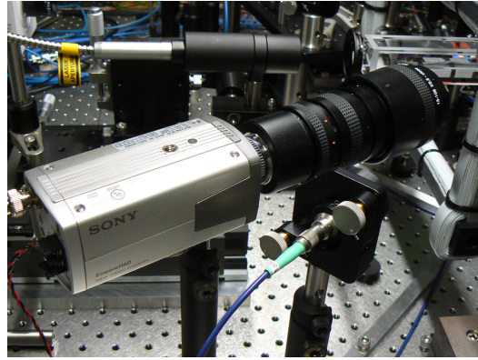
FIGURE 3.28: The CCD camera with zoom lens to monitor the atomic clouds.
