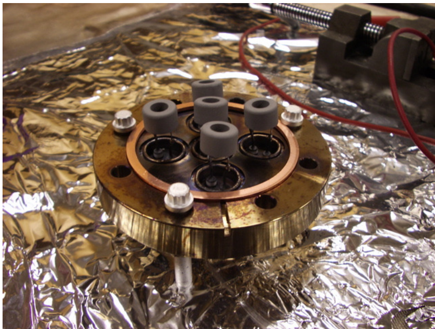
FIGURE 3.9: The getter pumps welded on the flange.
